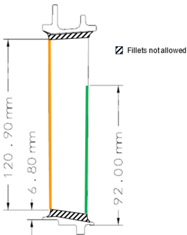
Figure 8. Cutbacks allowance areas.
