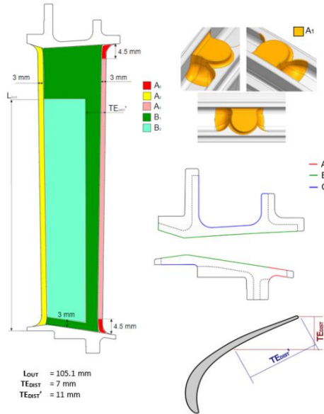
Figure 6. Defect zones (All dimensions in mm).
