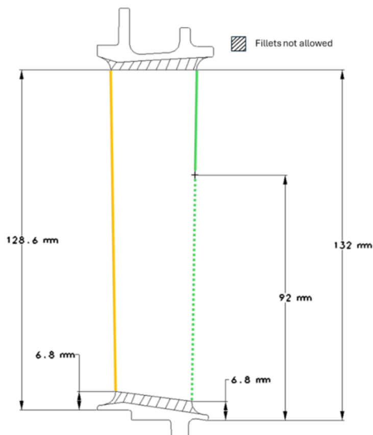
Figure 8. Cutbacks allowance areas.
