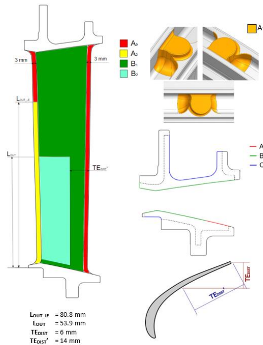
Figure 6. Blending allowance areas.
